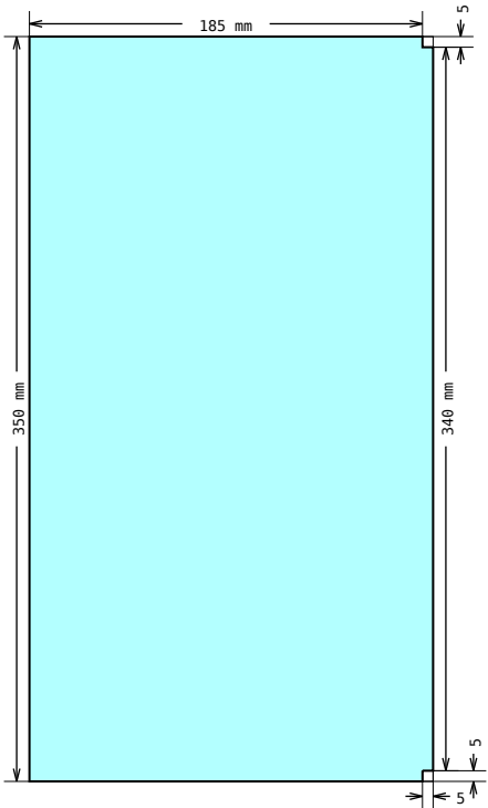
DRAWING 11, Pos 29 Shape measurements
