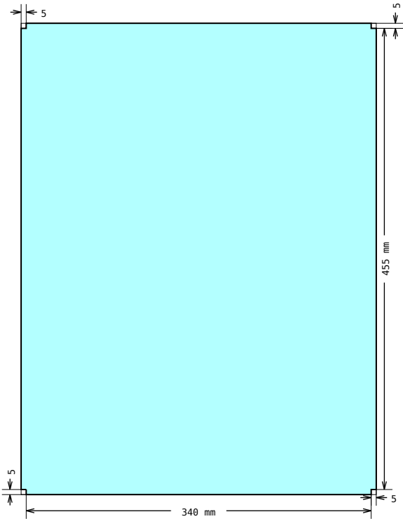
DRAWING 4, Pos 22 Shape measurements
