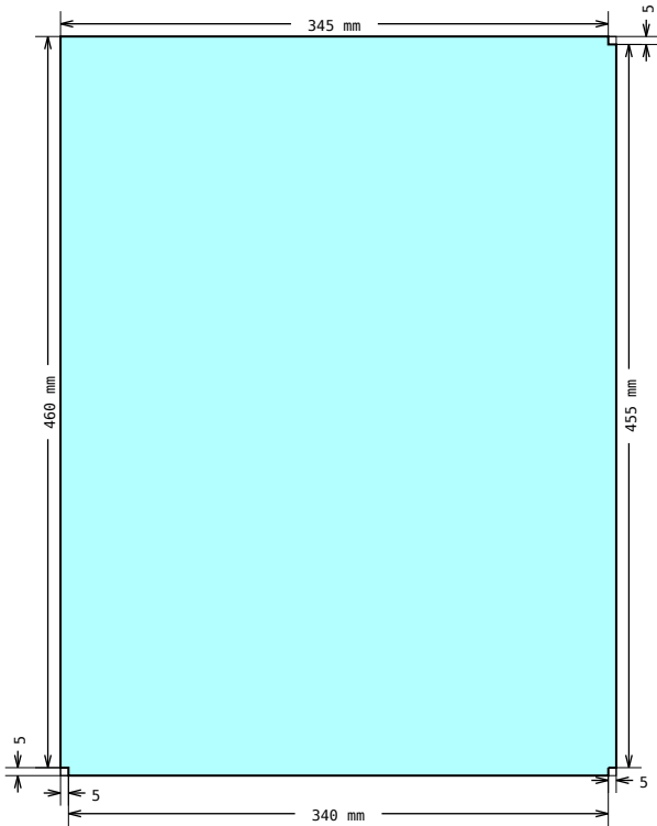
DRAWING 9, Pos 27 Shape measurements
