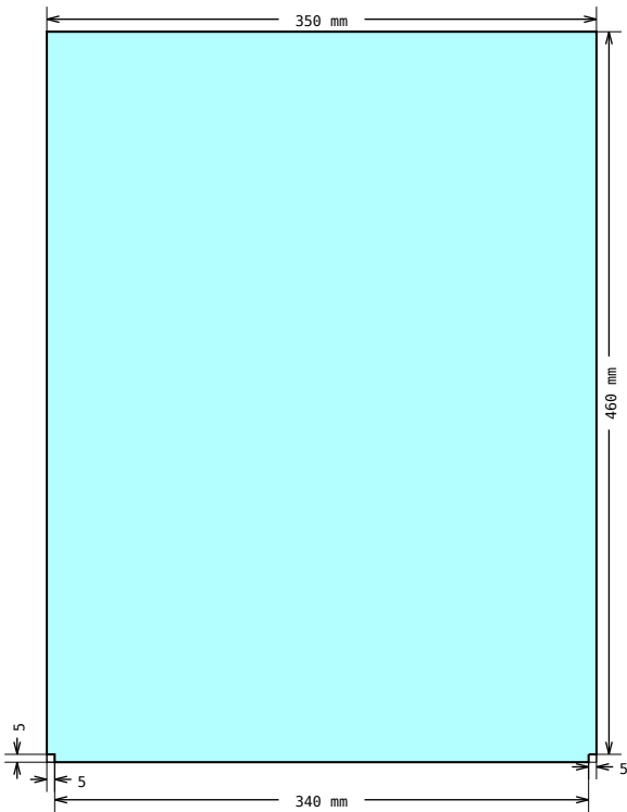
DRAWING 8, Pos 26 Shape measurements
