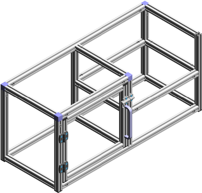
ISOMETRIC
