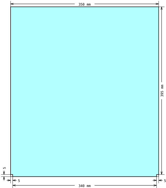
DRAWING 7, Pos 25 Shape measurements
