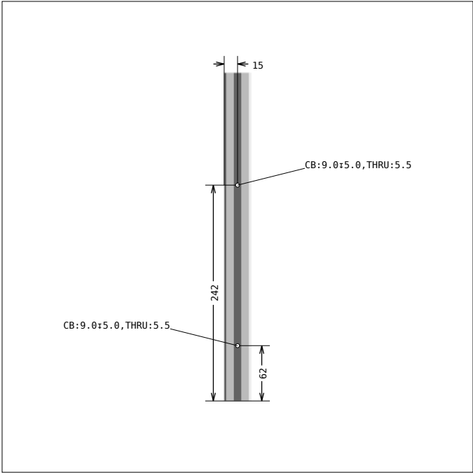
DRAWING 1, Pos 5 SIDE 4
