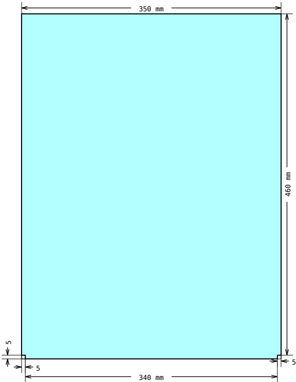
DRAWING 3, Pos 21 Shape measurements
